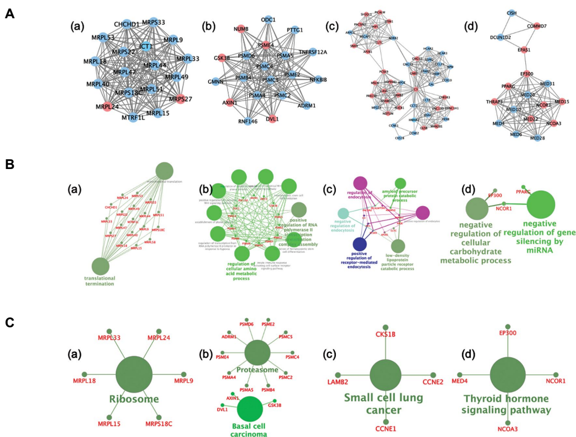
Fig.S1: Protein-protein interaction (PPI) network modeling. A. The top highly connected module (score>8) identified by MCODE. B, C. GO and KEGG analyses of the modules by ClueGo.
