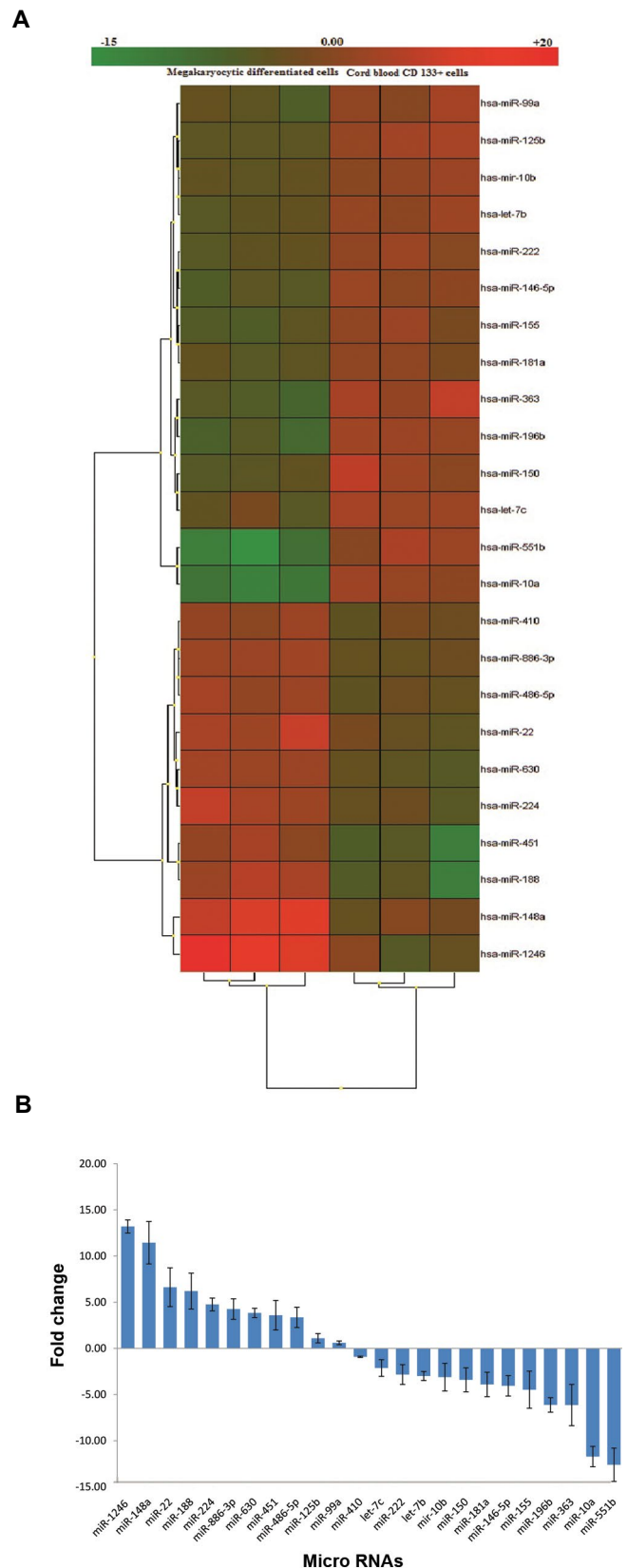
Fig.4: Alteration of miRNAs during megakaryocytic differentiation of CD133+ hematopoietic stem cells. A. Hierarchical clustering of 24 miRNAs by microarray analysis and B. Fold change expression of miRNAs by real time polymerase chain reaction (PCR).
