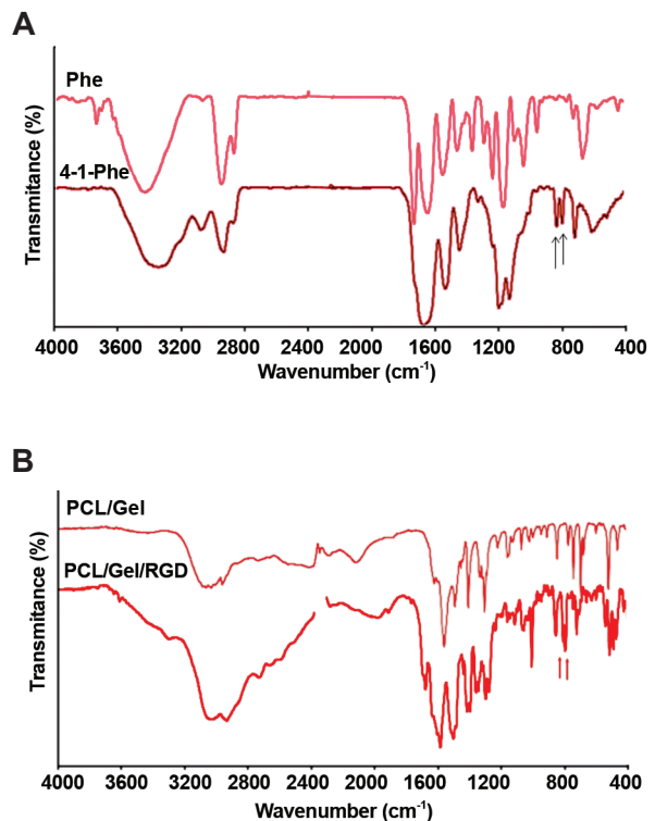
Fig 4: A. Fourier transform infrared spectroscopy (FTIR) of Phe and 4-Iodo-Phe standards. Arrows show the characteristic peaks assigned to C-I bond stretching. B. FTIR spectroscopy of PCL/Gel and RGD modified PCL/Gel. The assigned peaks are close to 800\text{ cm}^{-1} on the RGD modified PCL/Gel scaffold spectrum.
